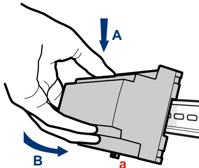
Abb. 3: Top-hat rail installation
