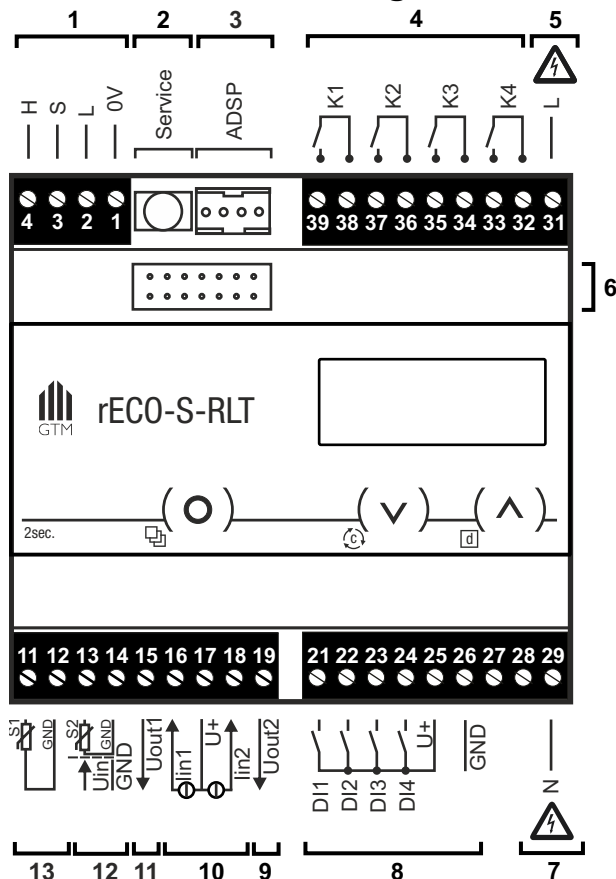
Abb. 2: Connection diagram
