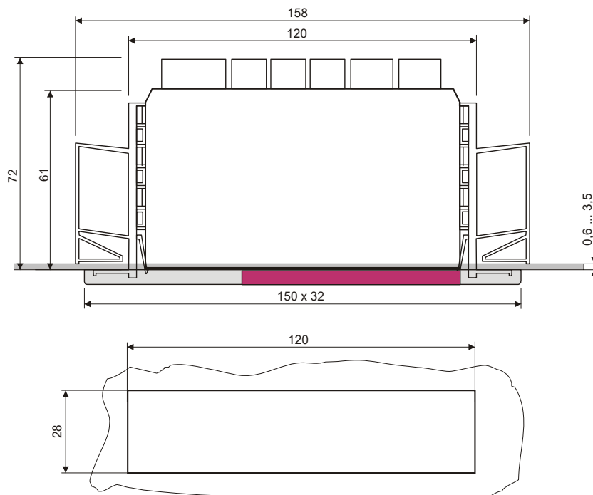
Installation section
