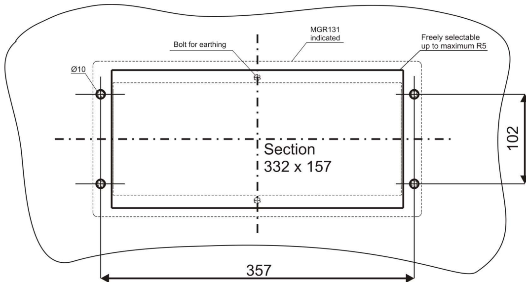
Fig. 3: Installation section MGR131 (all dimensions in mm)
