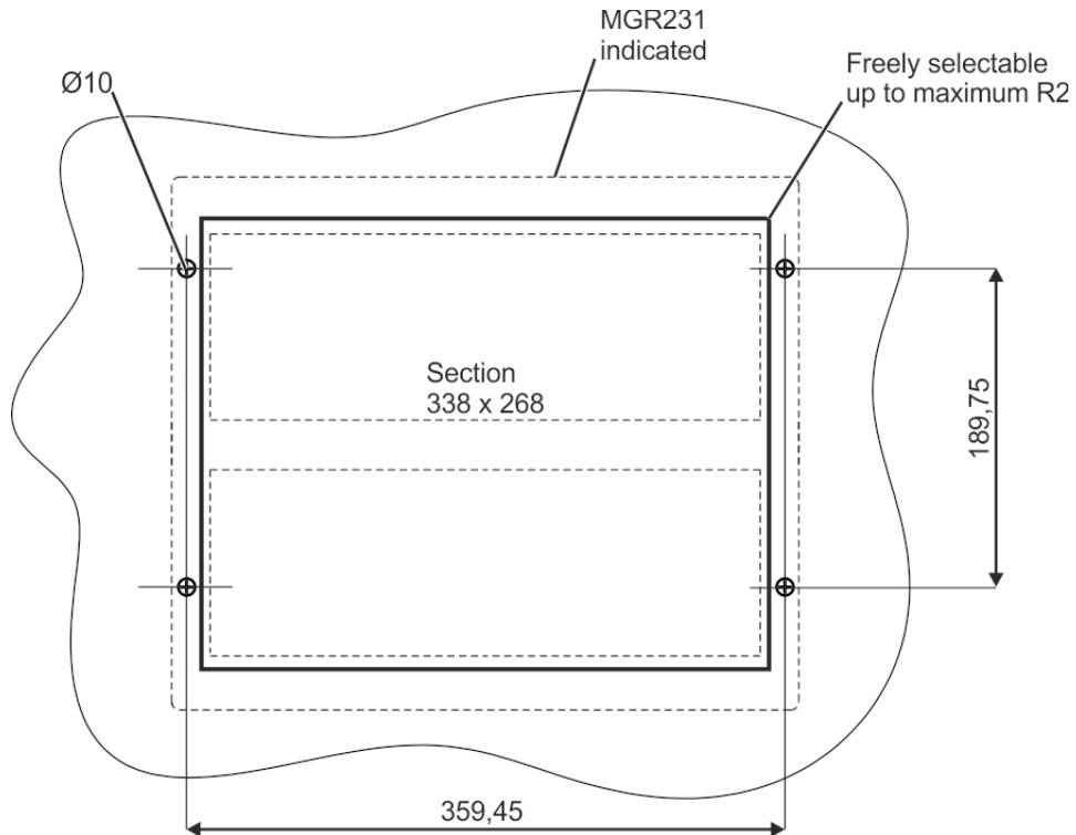
Fig. 5: Installation section MGR231 (all dimensions in mm)
