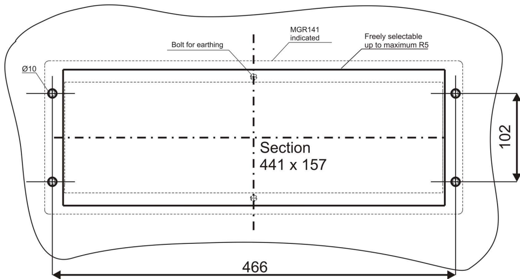
Fig. 4: Installation section MGR141 (all dimensions in mm)
