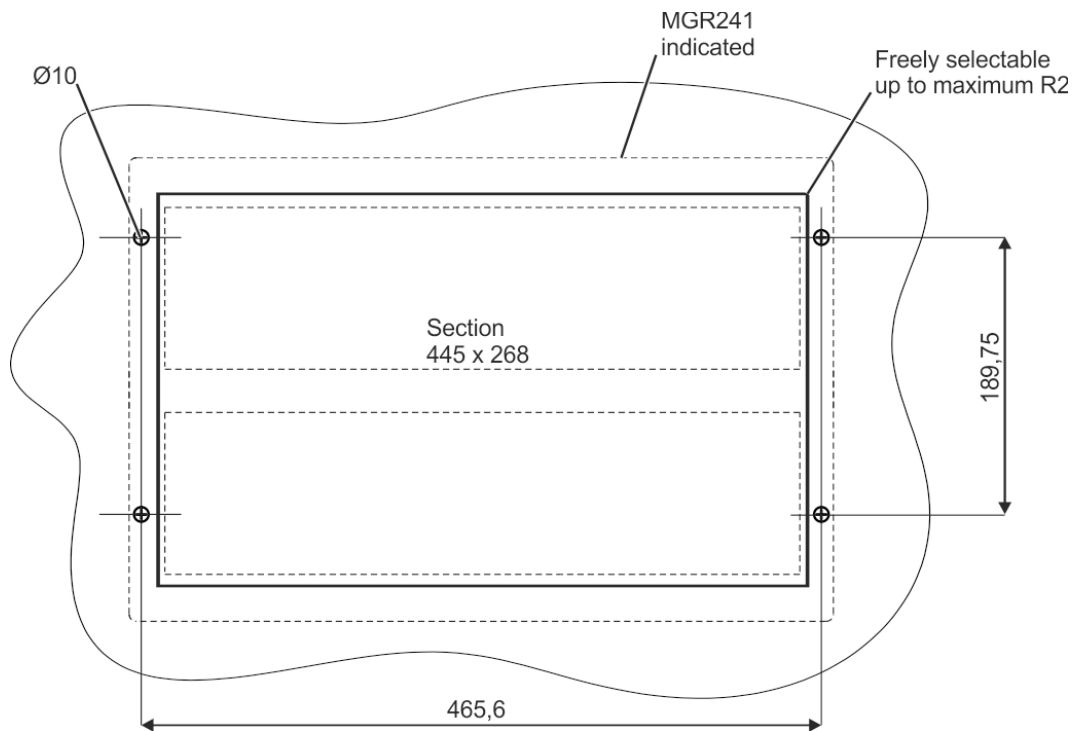
Fig. 6: Installation section MGR241 (all dimensions in mm)
